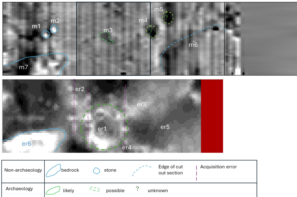
Figure 22: results of the Gradiometer survey (top) and ER (bottom). Colour scales as previous figure
