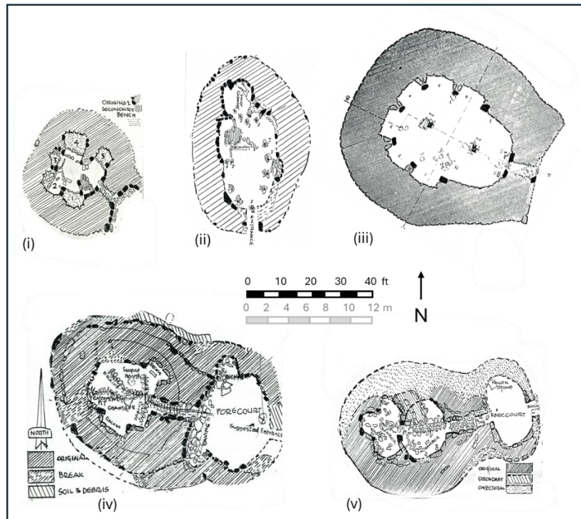
Figure 7: Ne/BA houses (i) Punds Water II (Calder 1968) (ii) House No.1 Gruting school, (Calder 1955/56 (iii) Stanydale, Crown Copyright: HES (Records of the Ordnance Survey Archaeology Division, Edinburgh, Scotland) (iv) Benie Hoose, Pettigarth Field Crown Copyright: HES (Records of the Ordnance Survey Archaeology Division, Edinburgh, Scotland) (v) Standing stones of Yoxie (Calder 1960/61)
