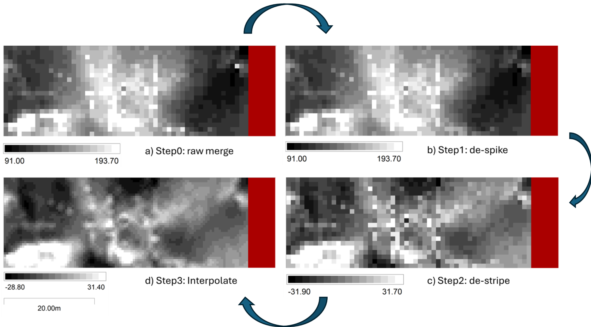
Figure 18: Uyea ER Data and processing results
